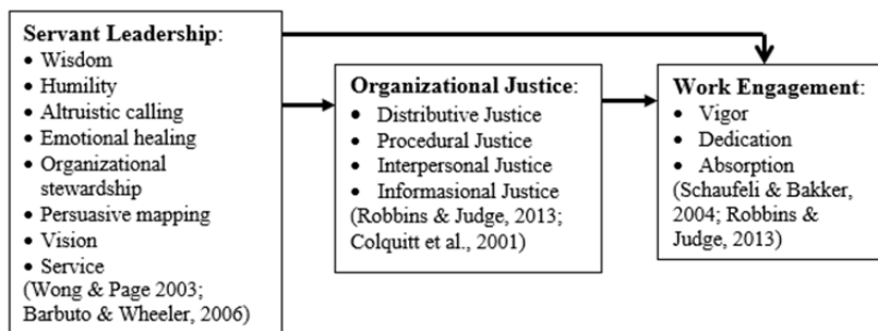
Figure 1: Conceptual Model
