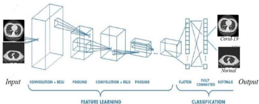
Gambar 3. Arsitektur Convolutional Neural Network (CNN)
