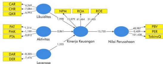
Fig 1. Summary of Statistical Calculation Results
