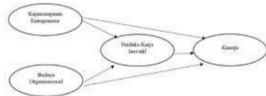
Gambar 1. Model Konseptual
