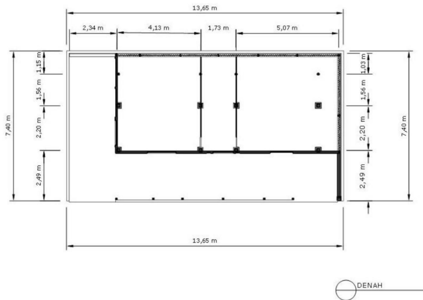
Figure3. Taneyan Lanjhang house building plan Source: Research team, 2023
