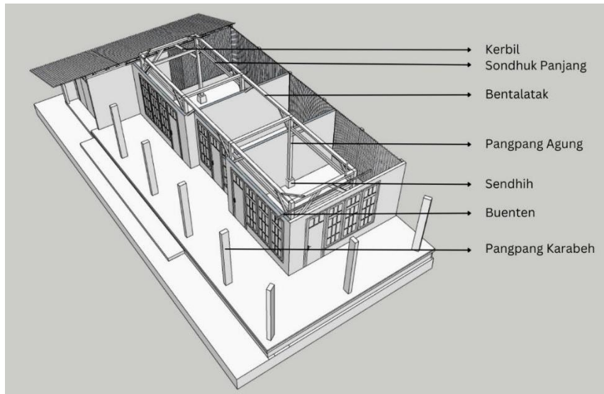
Figure6. Modern Madurese house building structure Source: Research team, 2023
