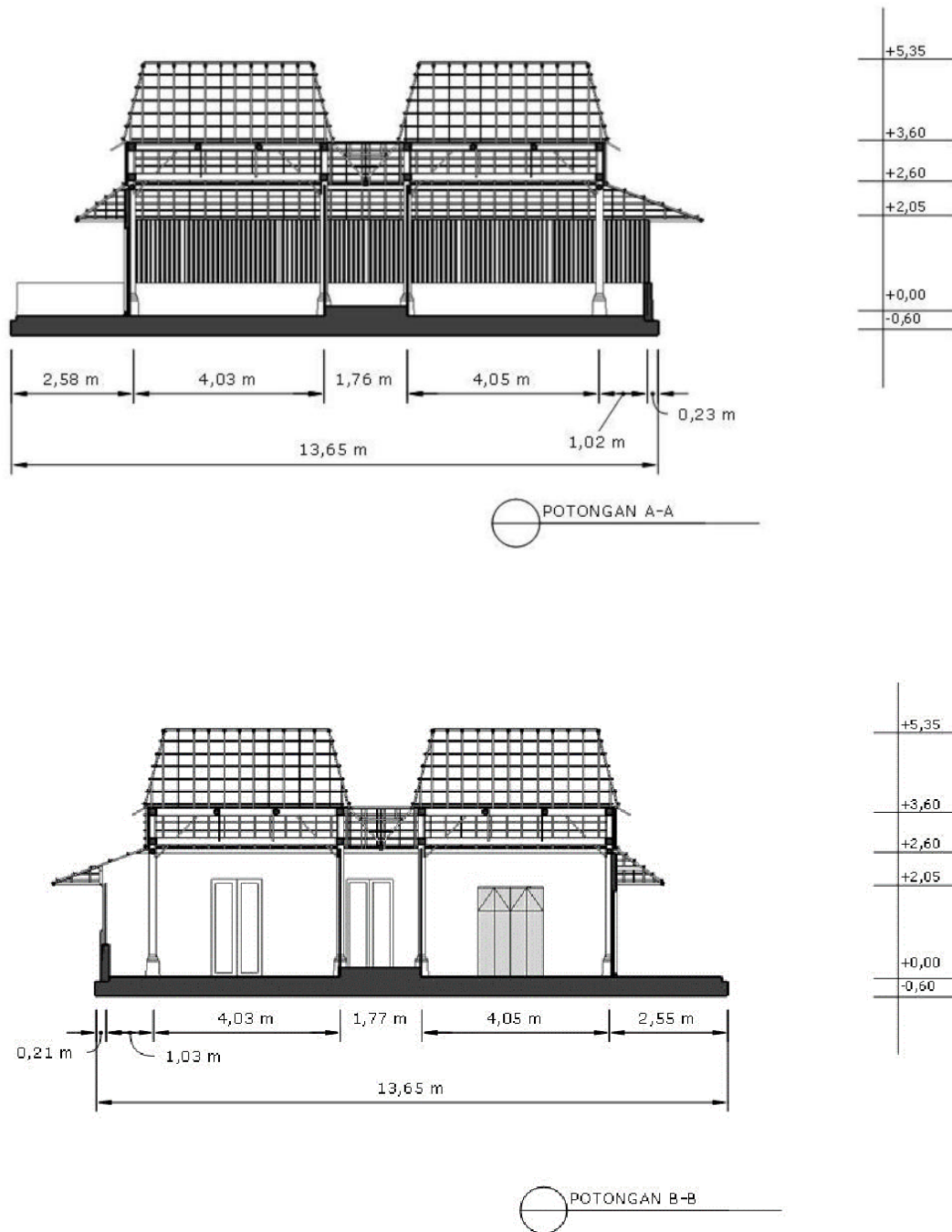
Figure4. Section of the Taneyan Lanjhang house building
