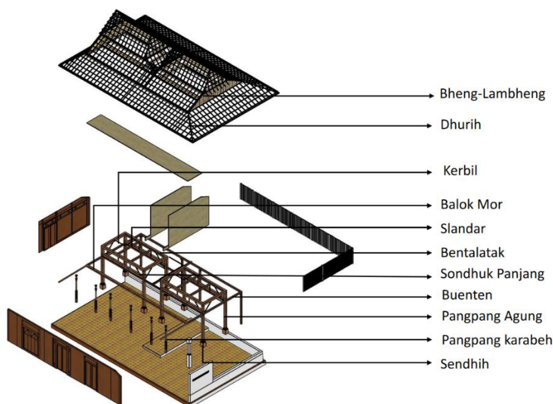
Figure1. Structure of Taneyan Lanjhang
