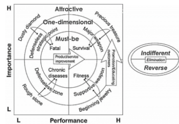
Fig. 2. IPA - Kano Method Integration Category Matrix
