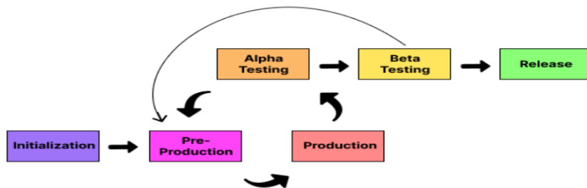
Fig.1 GDLC Flow
