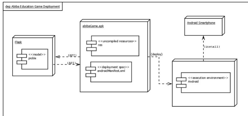
Fig.4 Deployment Diagram
