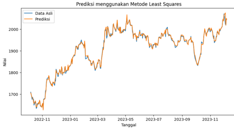
Gambar 3. Prediksi OLS (Least Square)
