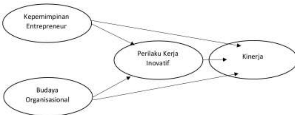
Gambar 1. Model Konseptual
