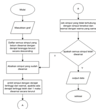
Gambar 5. Diagram Alir Algoritma Recursive Largest First
