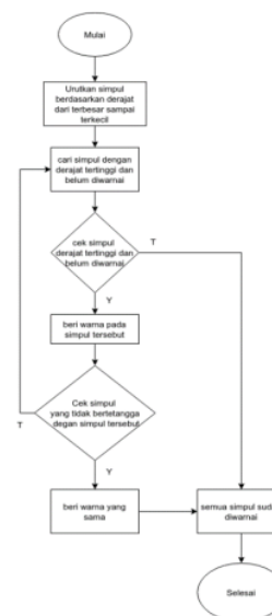
Gambar 4. Diagram Alir Algoritma Welch-powell
